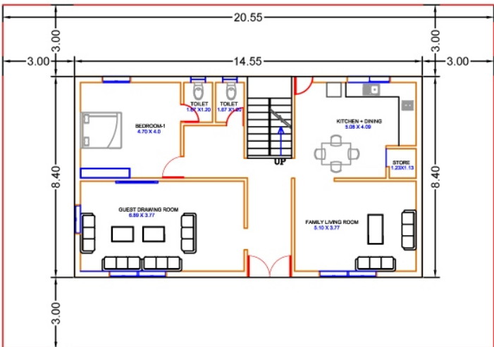
GROUND FLOOR (UNIT AREA- 295 SQMT)
