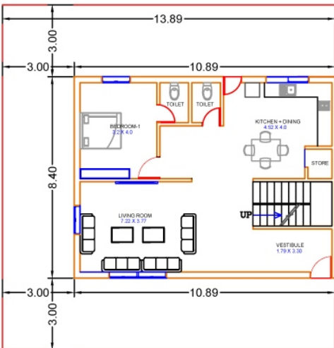
GROUND FLOOR (UNIT AREA- 200 SQMT)
