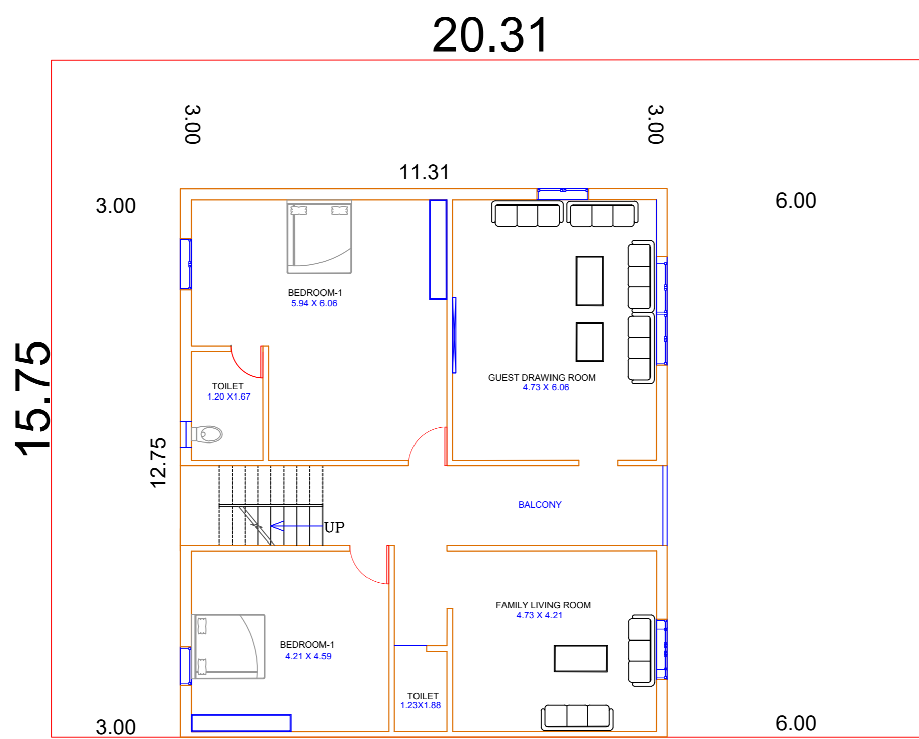
FIRST FLOOR
