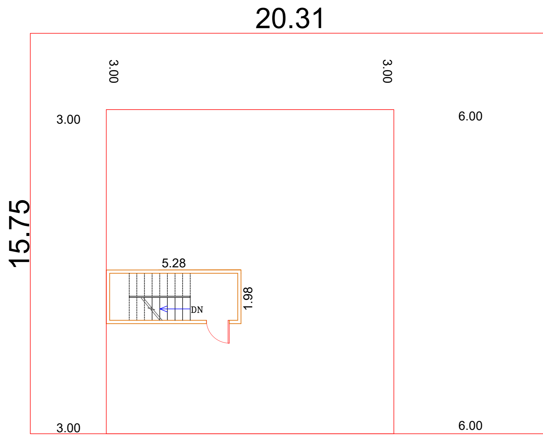
TERRACE FLOOR
