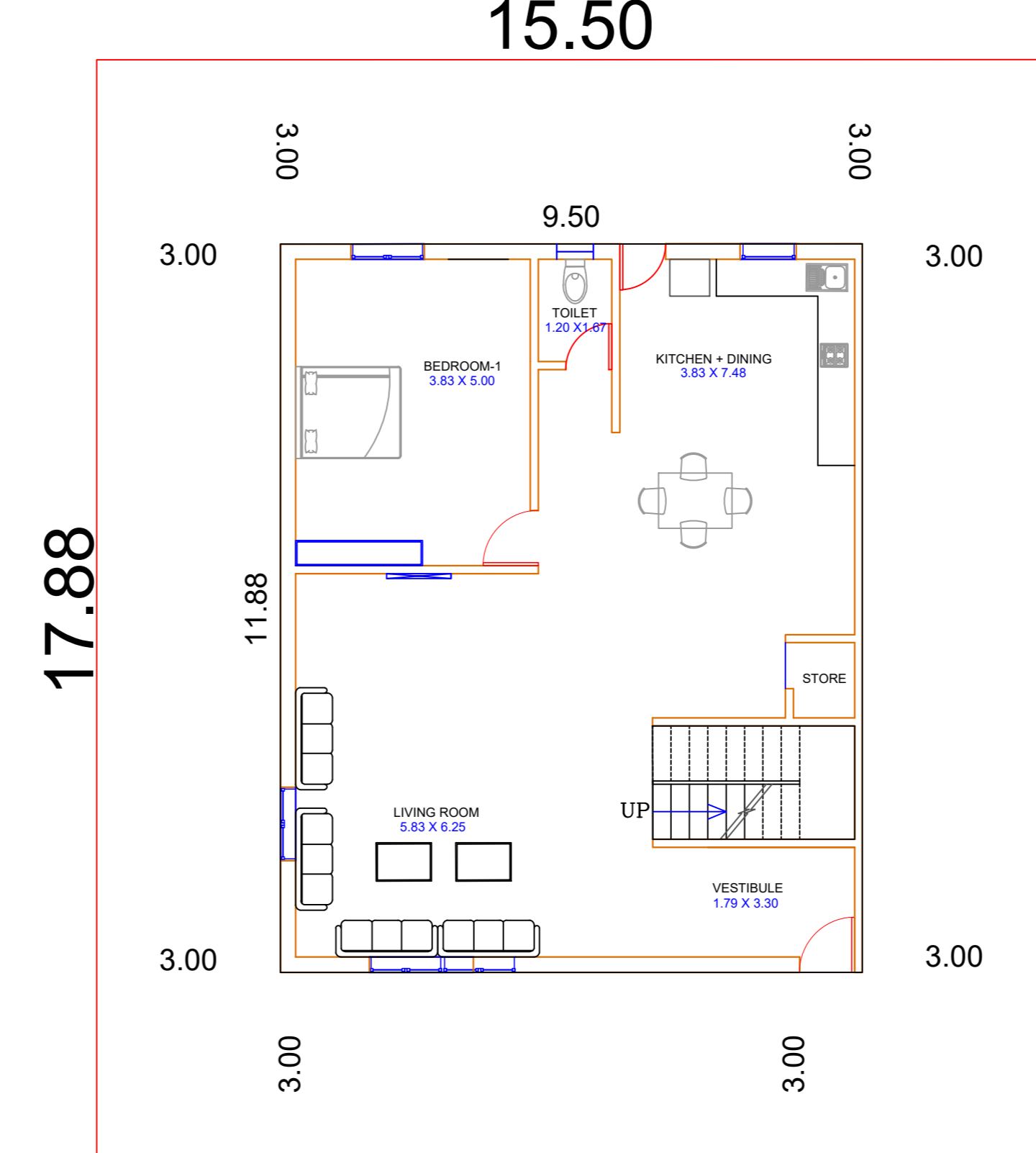
GROUND FLOOR (UNIT AREA- 277.14 SQMT)
