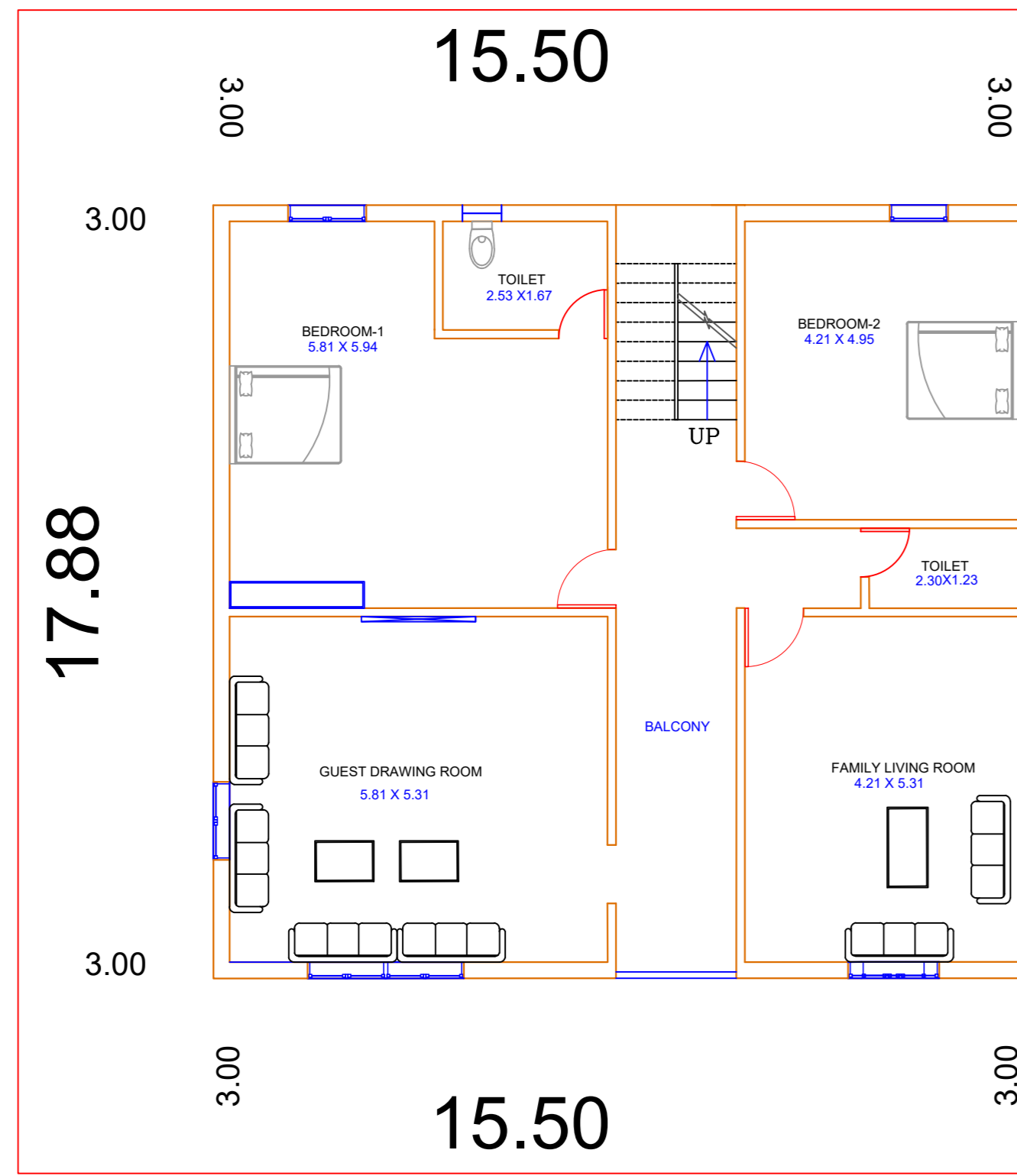
FIRST FLOOR
