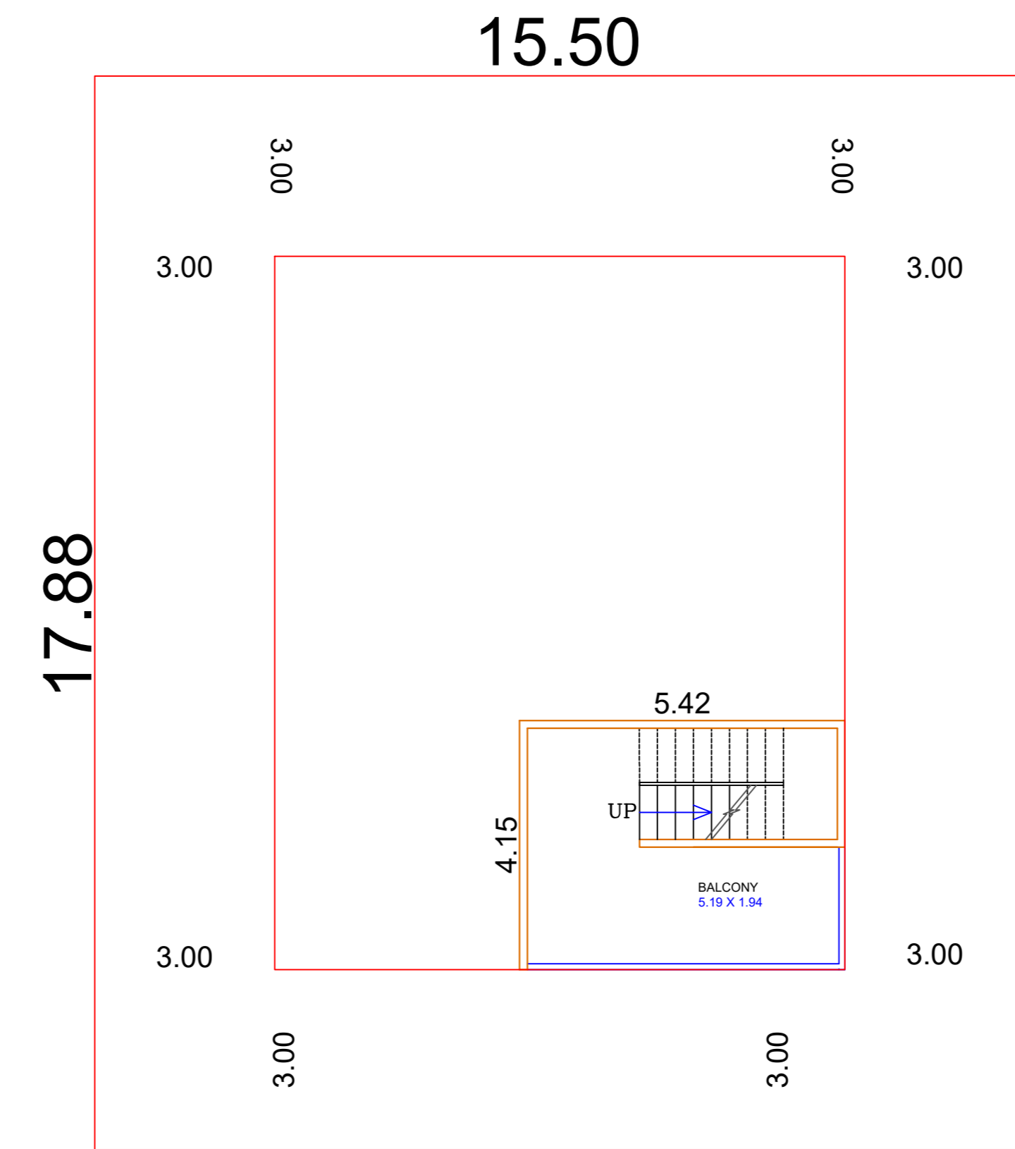
FIRST FLOOR
